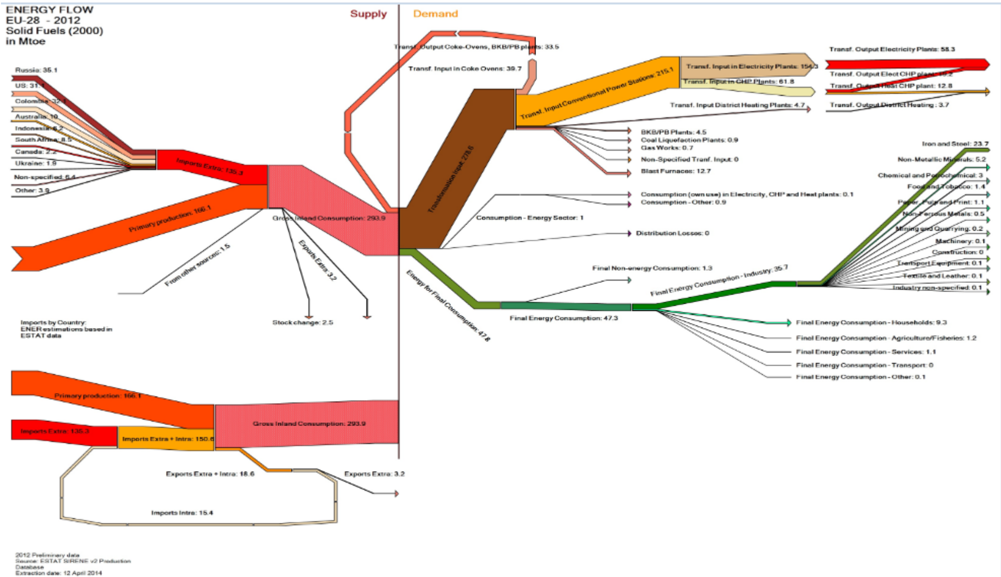
Figure 46. Energy flow of solid fuels in the EU, 2012
