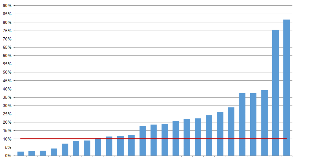
Figure 92 Ratio of available cross-border electricity interconnector capacities compared to domestic installed power generation capacities
